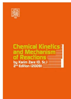
Chemical Kinetics and Mechanism of Reactions Karim Zare
